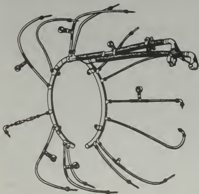
FIGURE 4-10. A high-tension ignition harness.
